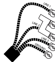
3 x 230 VAC (3 x 16A) Three-phase (Delta)
