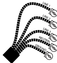
3 x 230 VAC (3 x 16A) Three-phase
